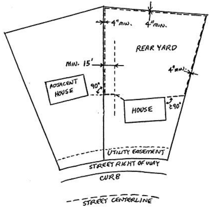
PERIMETER FENCING GUIDELINE illustrating avoiding front yard of adjacent house
